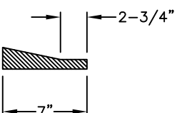
SECTION L-L
