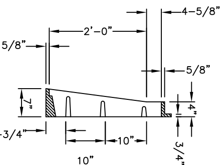
SECTION J-J
