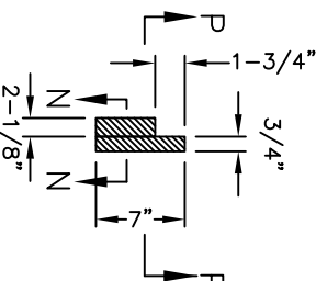
SECTION M-M
