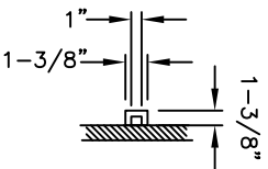
SECTION N-N
