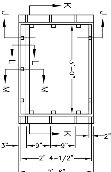
FRAME PLAN
