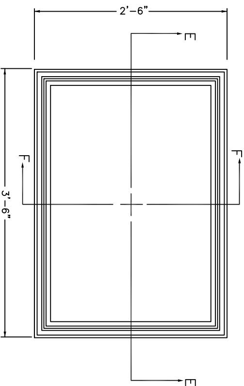
PLAN OF FRAME CAST IRON
