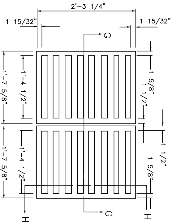
PLAN OF GRATING CAST IRON
