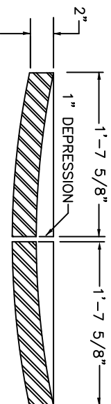
SECTION G-G
