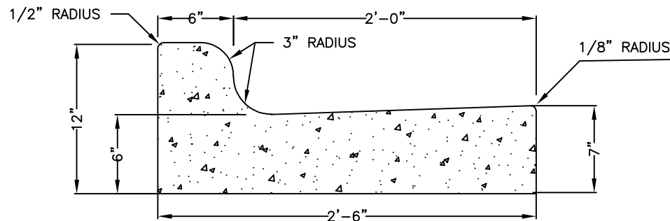
STANDARD 2'-6" CURB AND GUTTER
