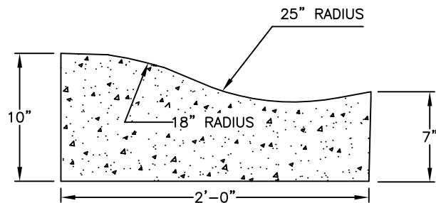
2'-0" VALLEY GUTTER
