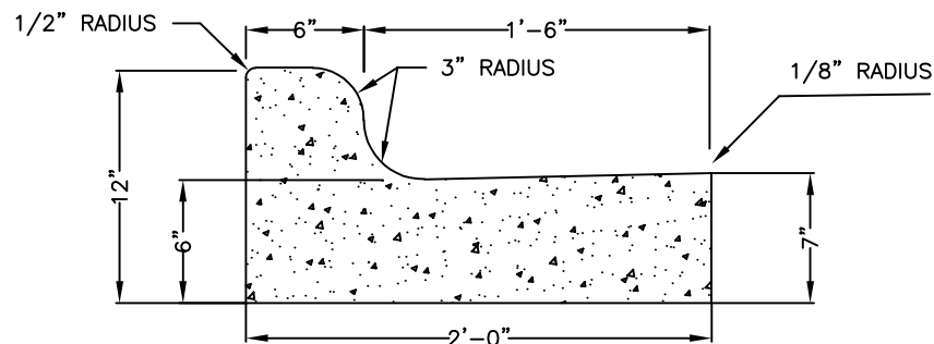
STANDARD 2'-0" CURB AND GUTTER
