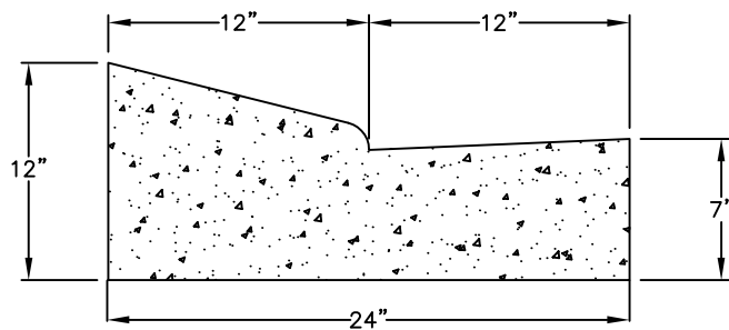
2'-0" MOUNTABLE CURB
