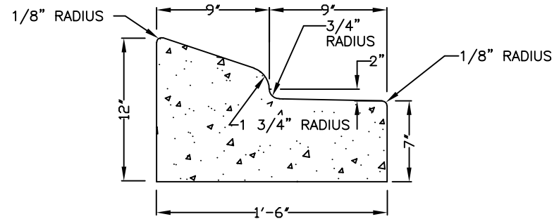
1'-6" MOUNTABLE CURB AND GUTTER FOR MEDIANS
