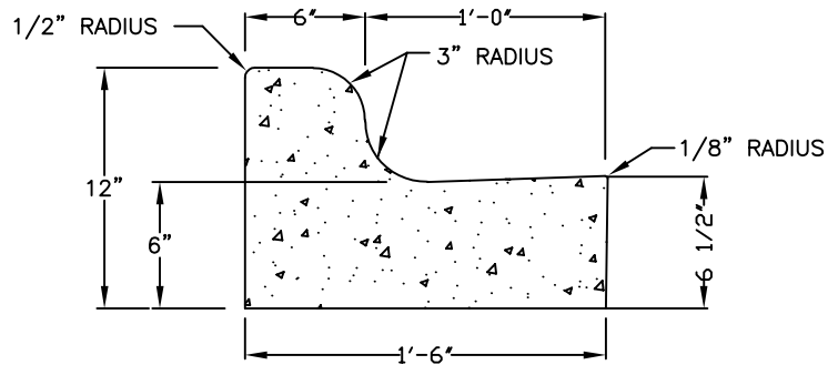
STANDARD 1'-6" CURB AND GUTTER
