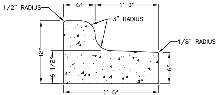
1'-6" MEDIAN CURB AND GUTTER FOR MEDIANS
