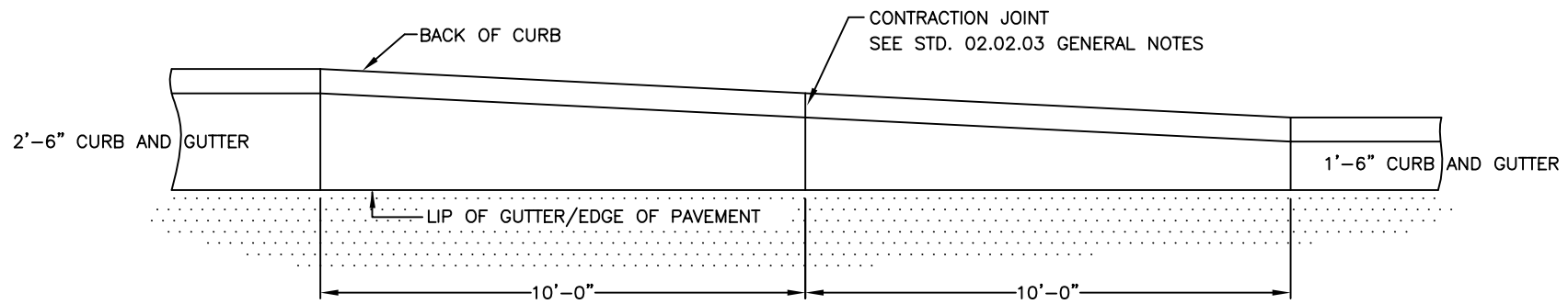
PLAN VIEW
